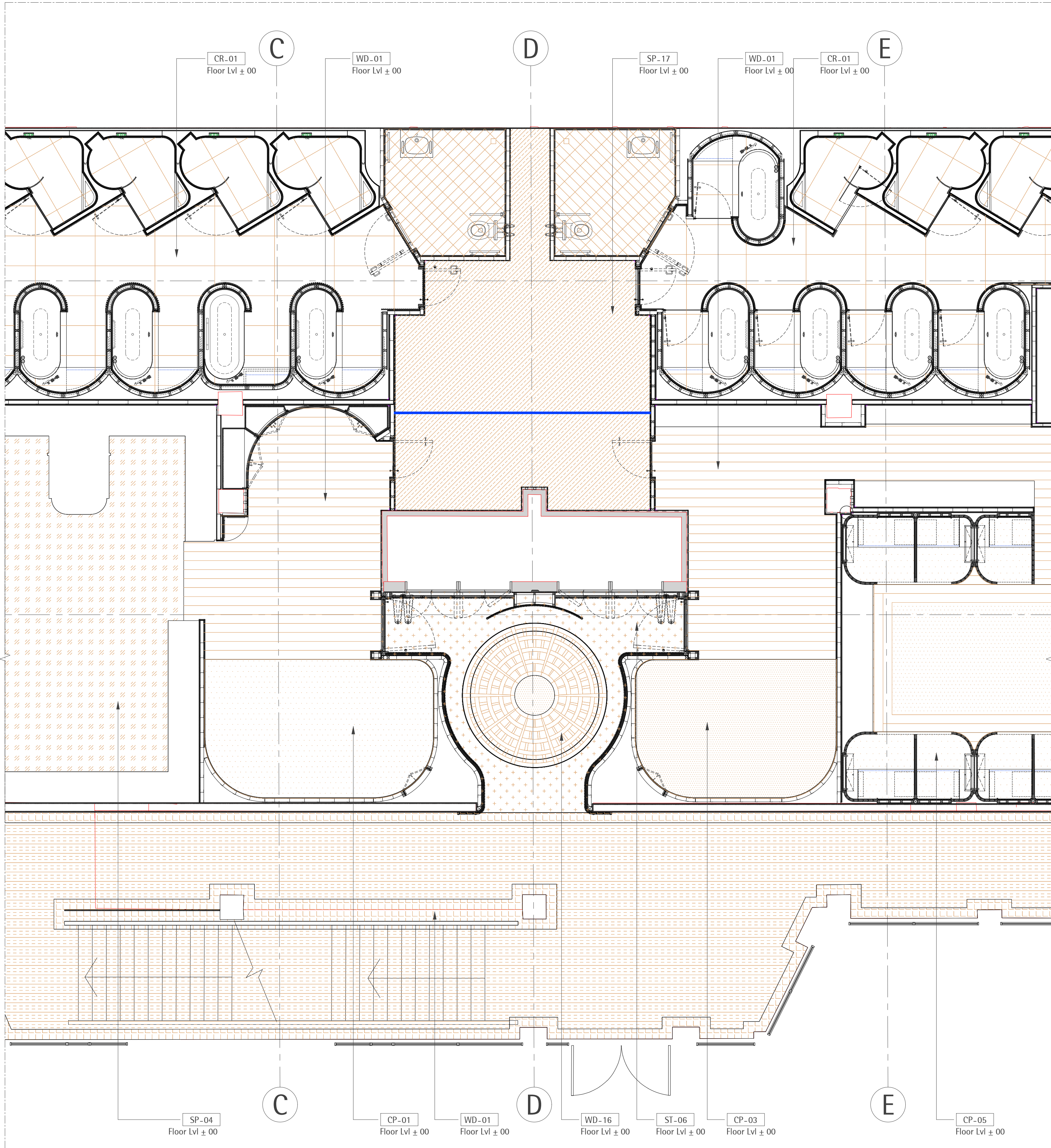
01 Floor Finishes SCALE 1:75
