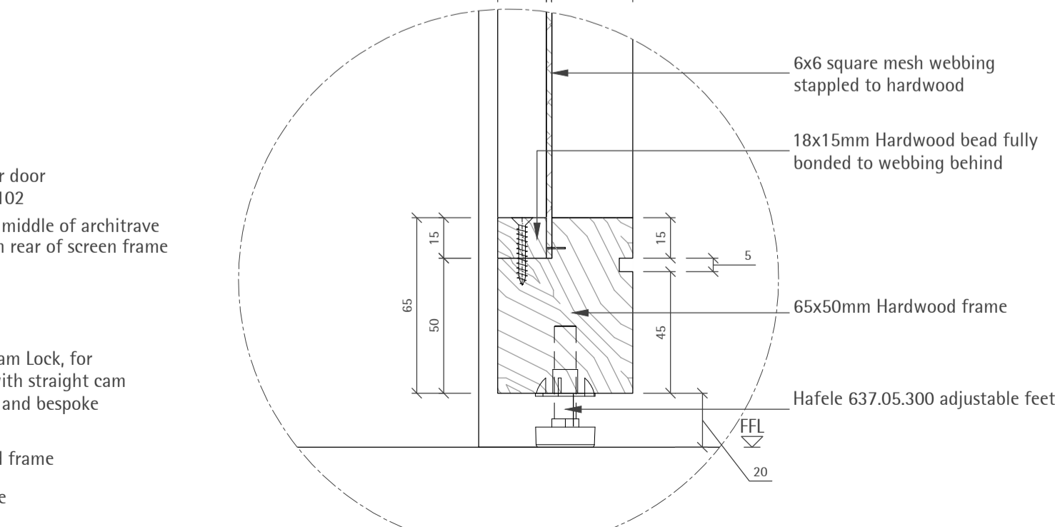
06 DETAIL SCALE 1:2
