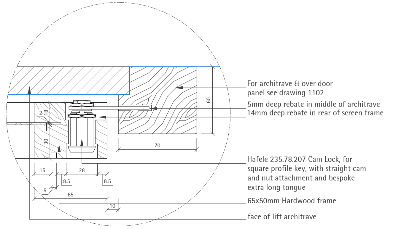
06 DETAIL SCALE 1:2
