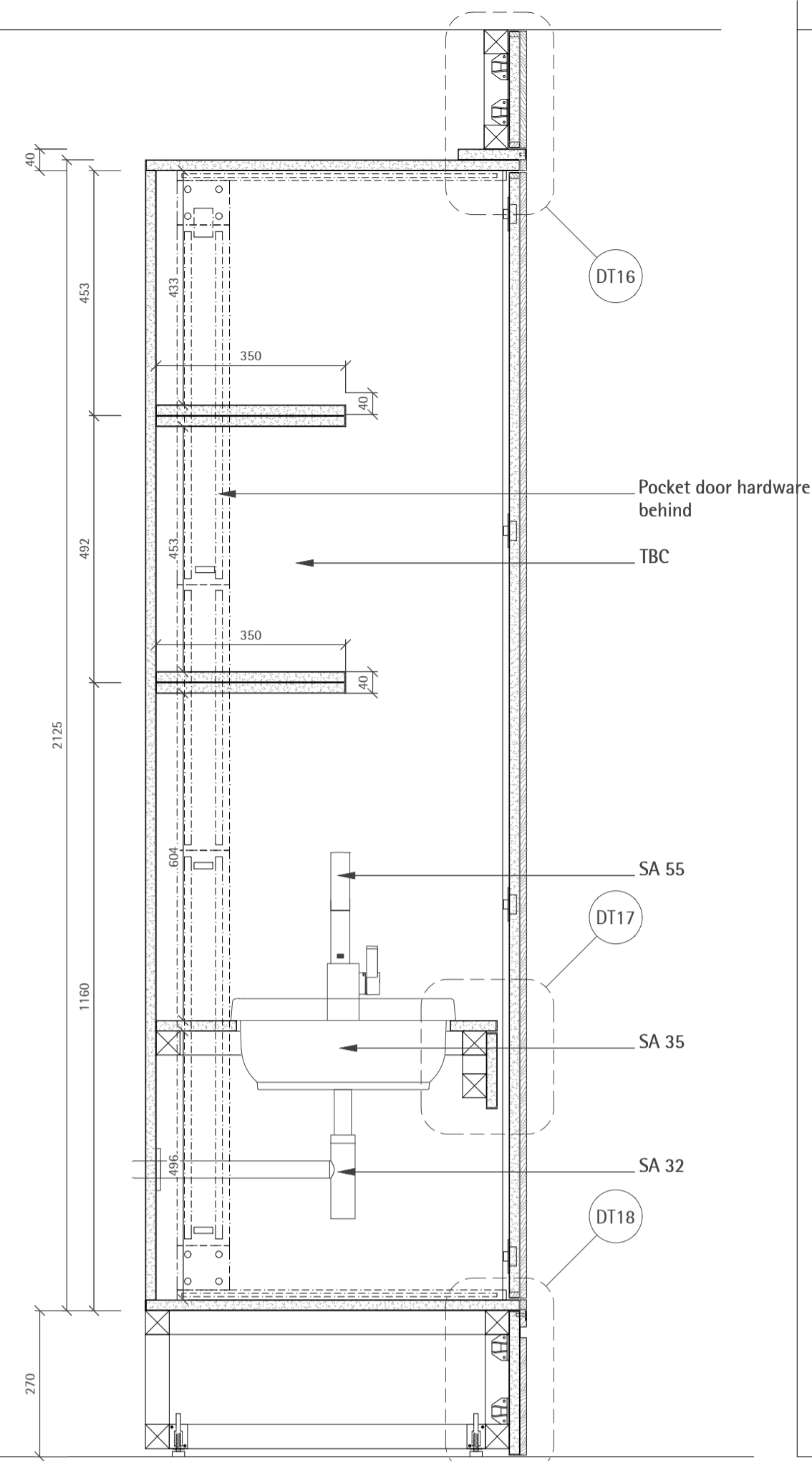
05 SECTION SCALE 1:10
