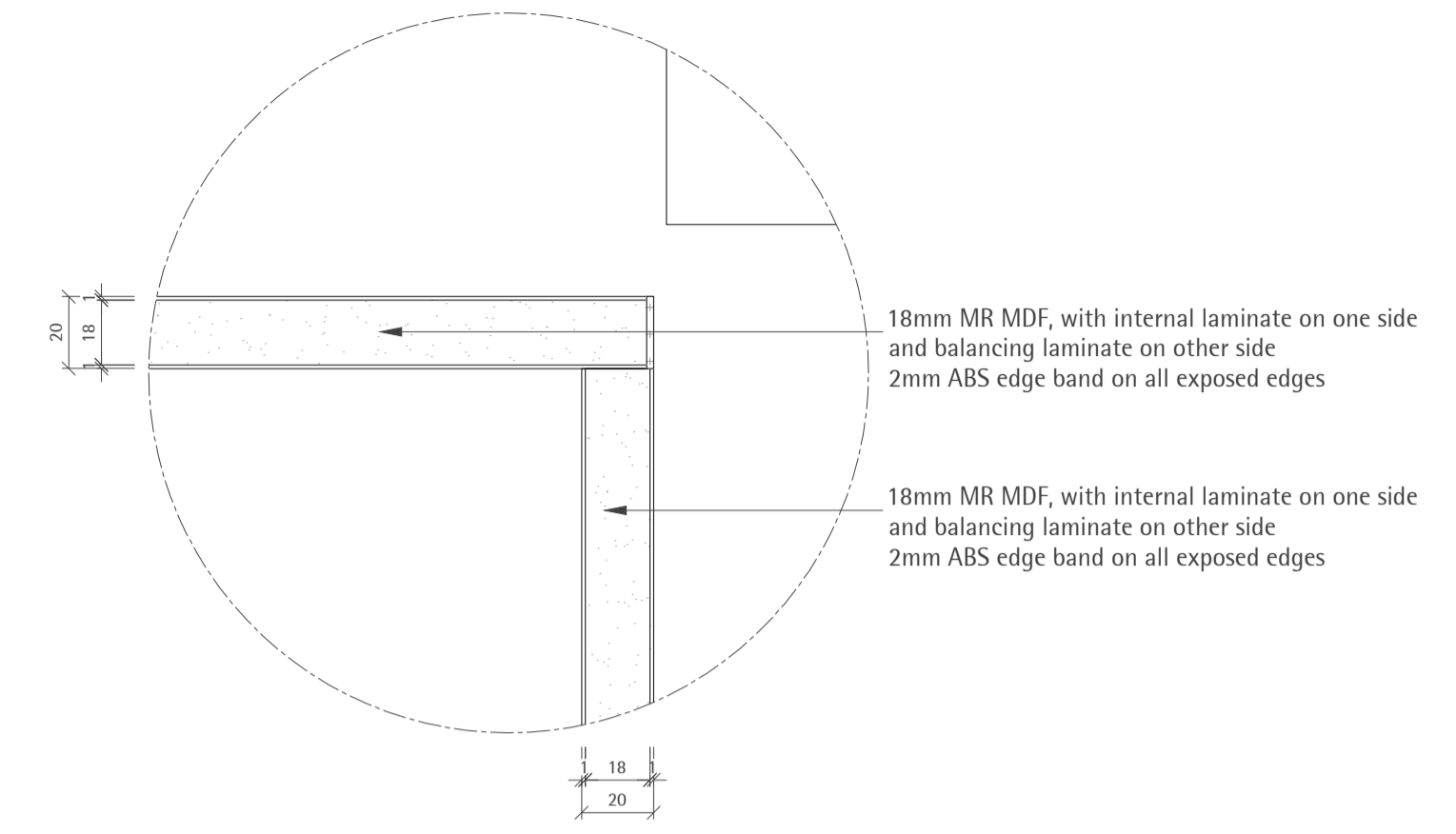
DT10 DETAIL SCALE 1:2
