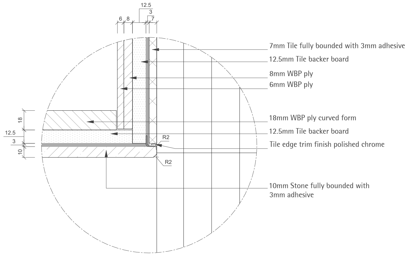
DT02 DETAIL SCALE 1:2
