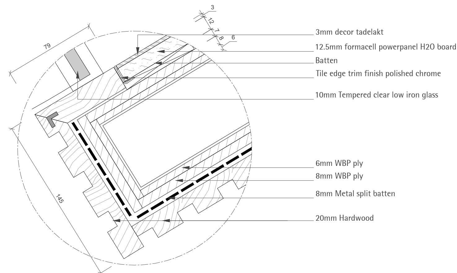
DT07 DETAIL SCALE 1:2
