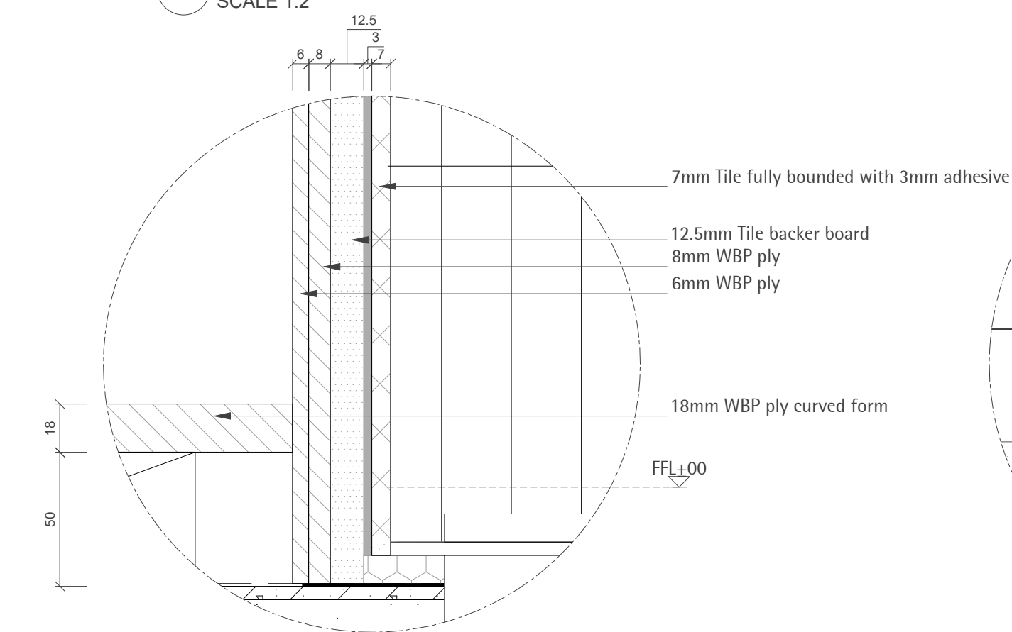
DT03 DETAIL SCALE 1:2
