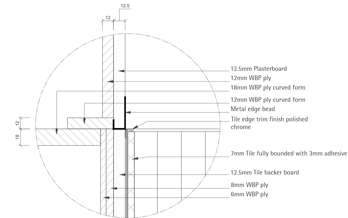
DT01 DETAIL SCALE 1:2
