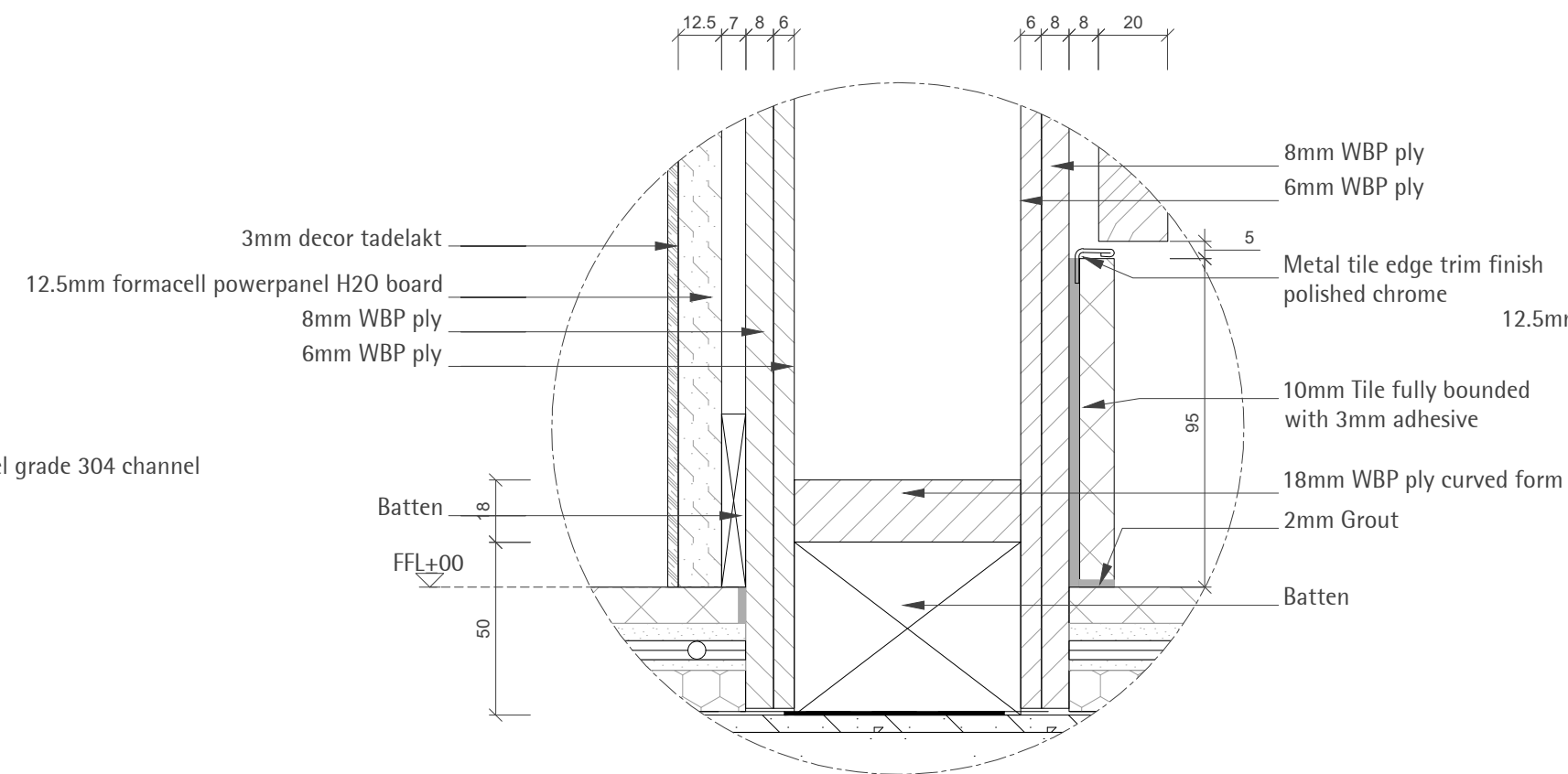
DT07 DETAIL SCALE 1:2
