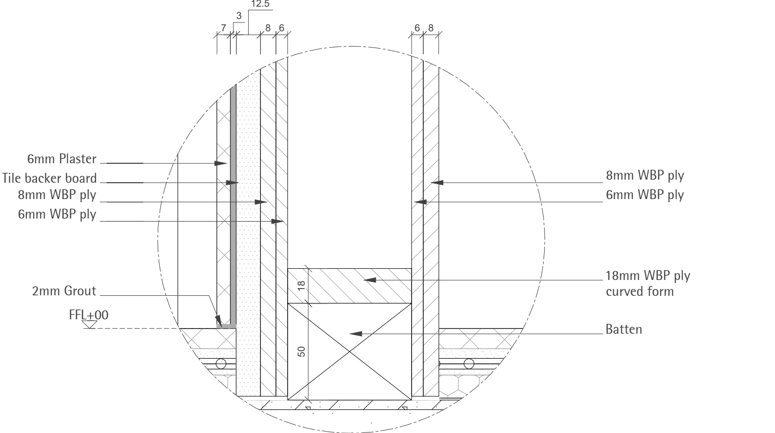
DT09 DETAIL SCALE 1:2
