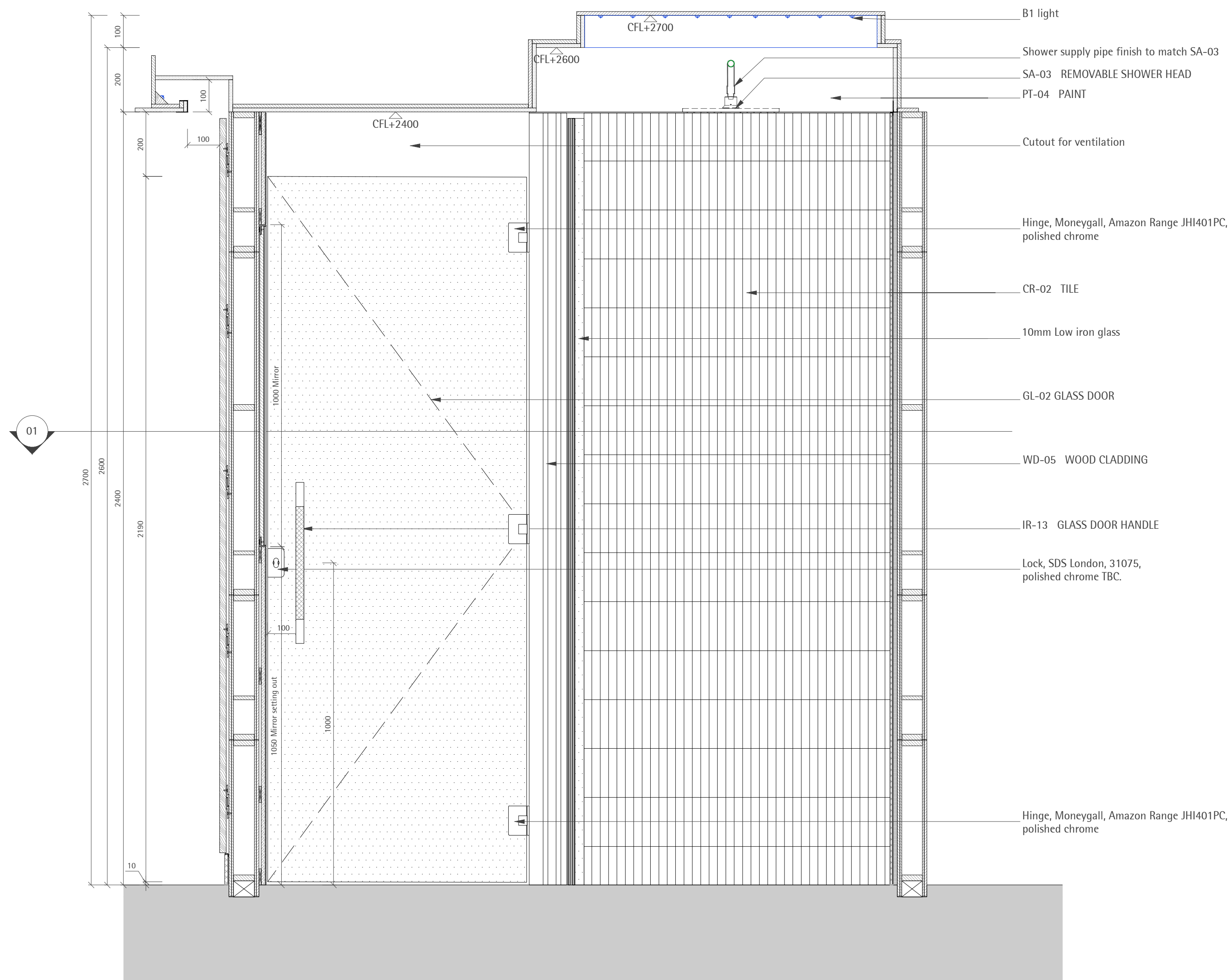
05 ELEVATION SCALE 1:10
