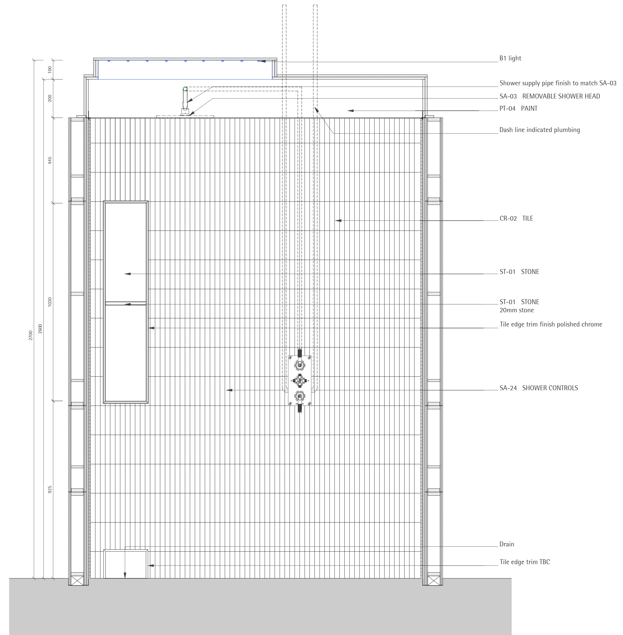
06 ELEVATION SCALE 1:10
