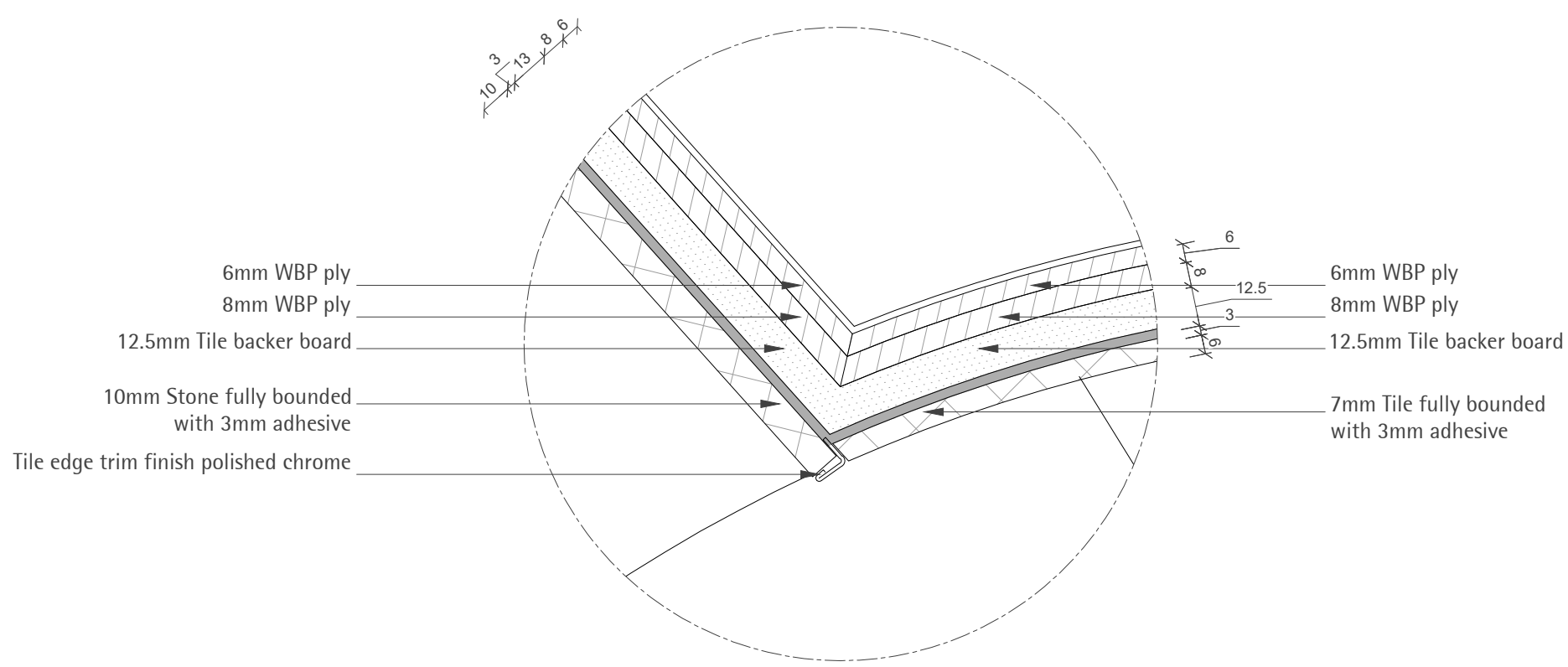
DT01 DETAIL SCALE 1:2
