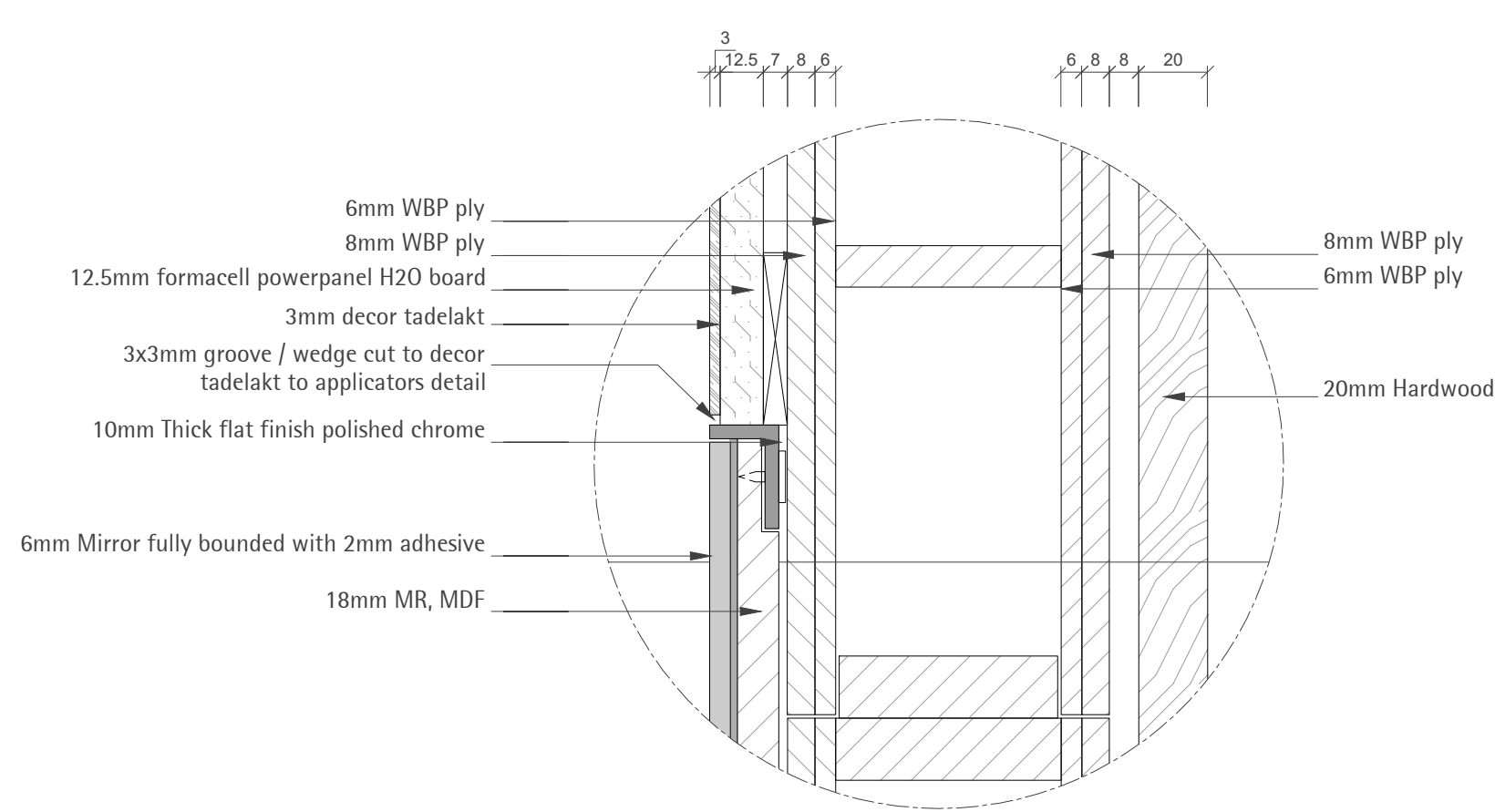
DT06 DETAIL SCALE 1:2
