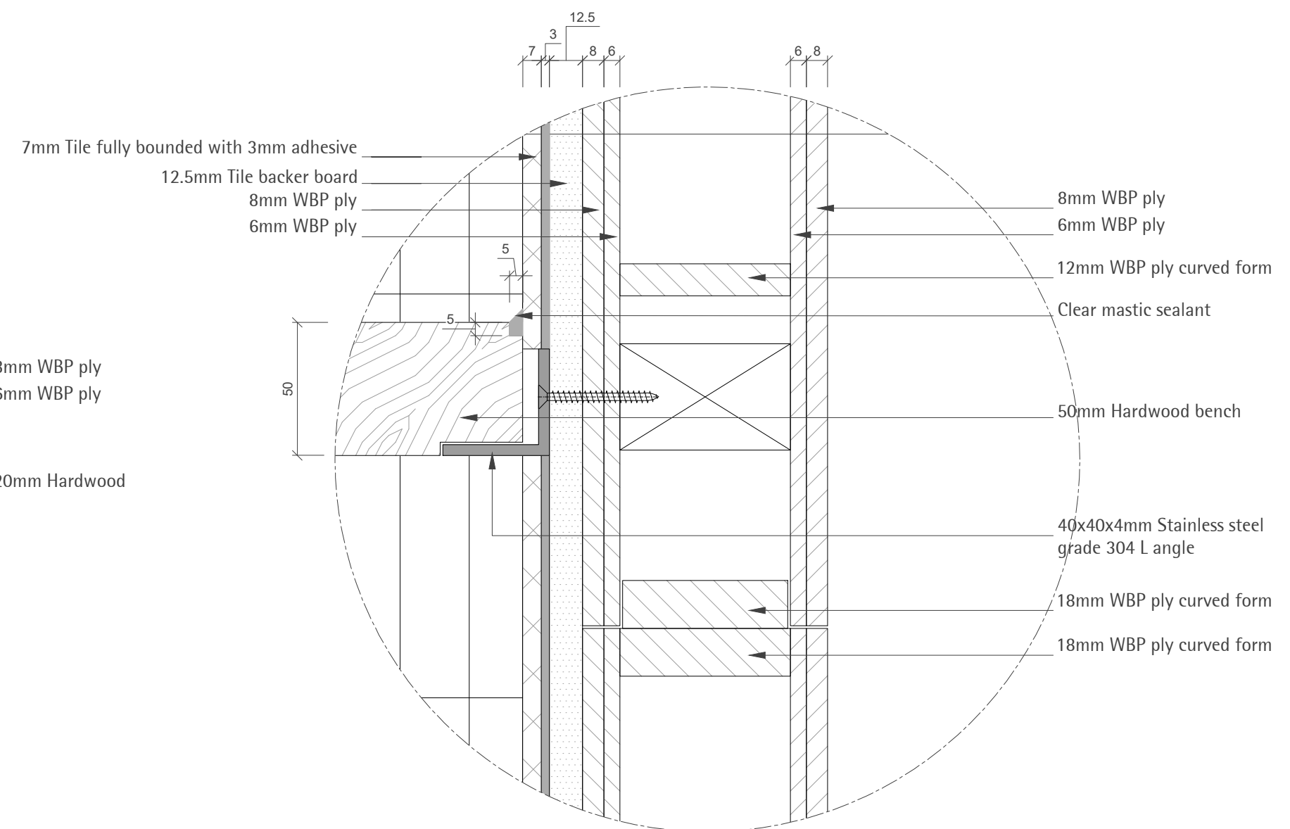
DT08 DETAIL SCALE 1:2
