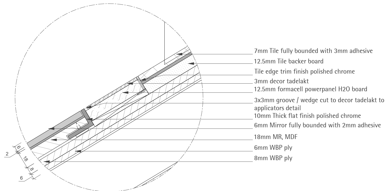
DT06 DETAIL SCALE 1:2
