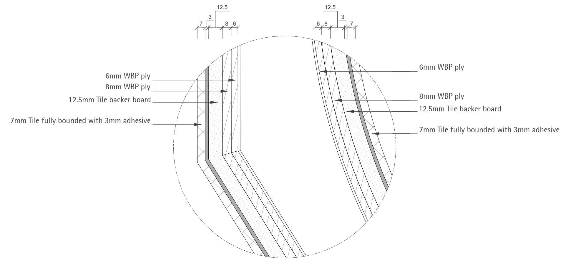
DT03 DETAIL SCALE 1:2
